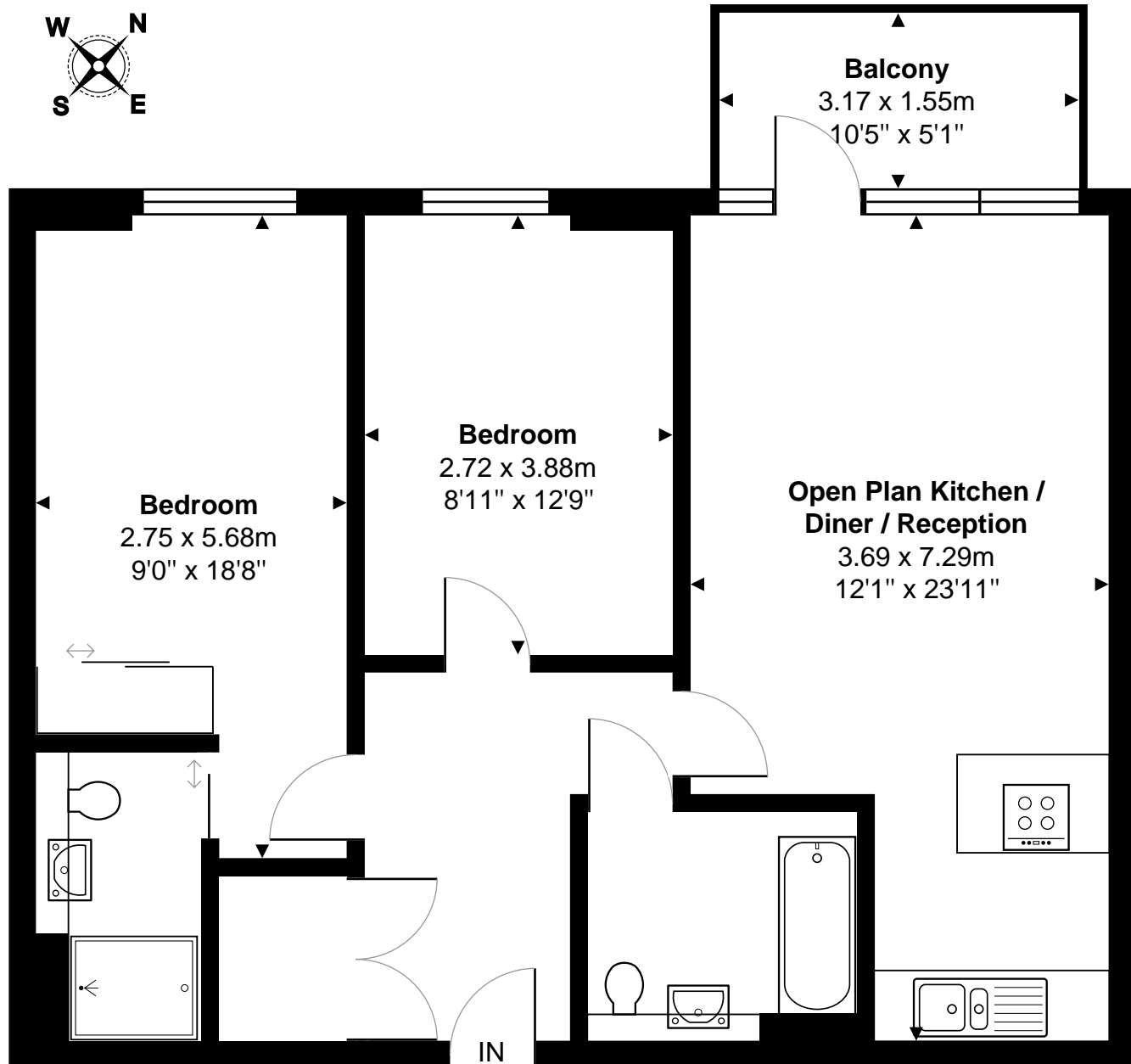
Fifth Floor
